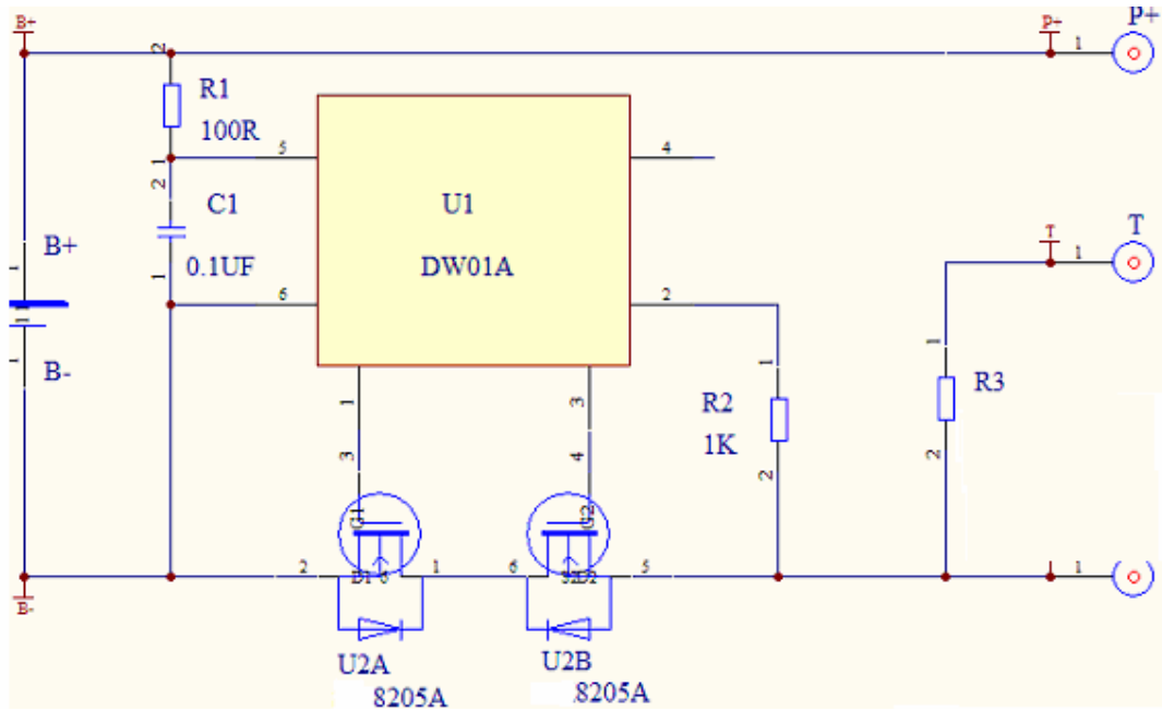
7.2.3 Application Circuit 线路板原理图
