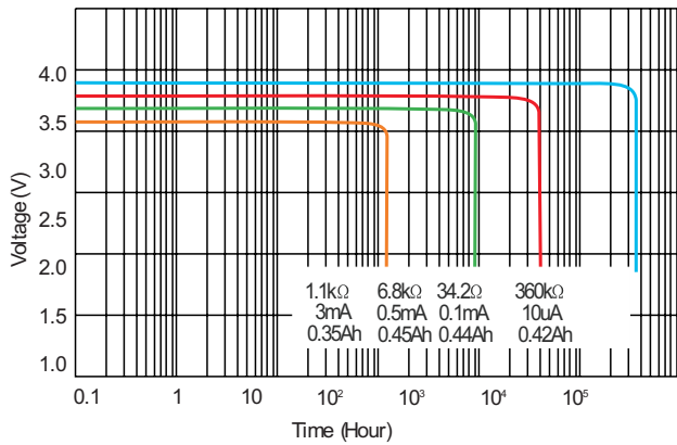
Voltage plateau versus Current and Temperature
