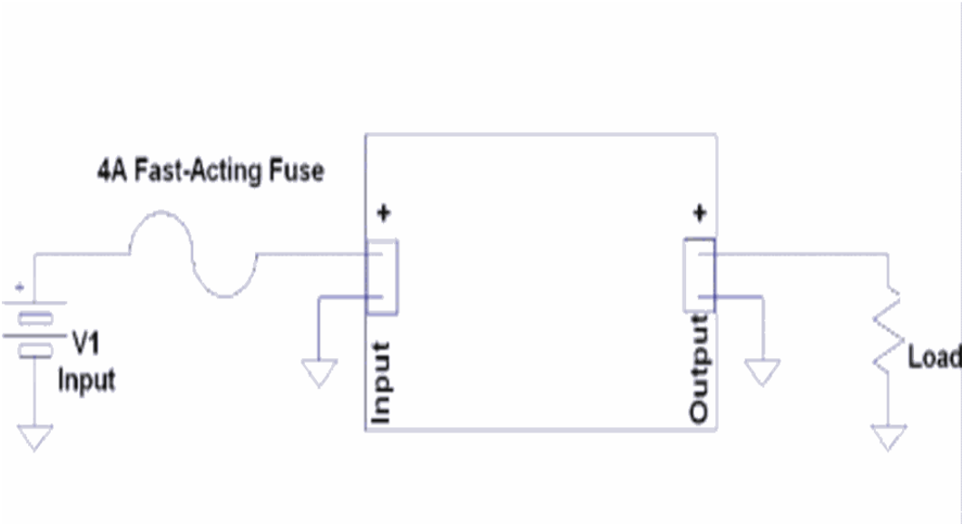
Figure 2 Connection diagram
