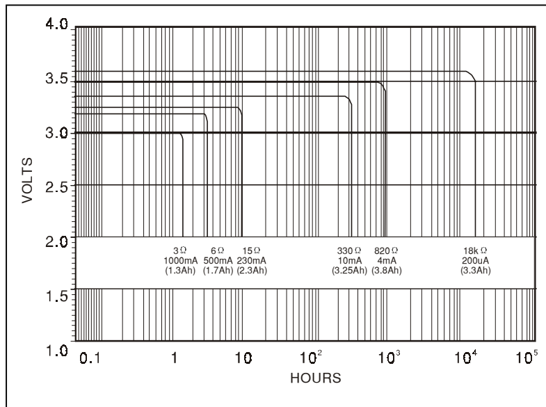
Capacity vs. Different discharging rate
